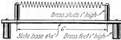
3 Coils each containing 5 ft. of No. 22 resistance wire. Wind 48 turns on \frac{3}{8} -in. rod
